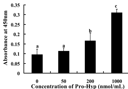
Figure 6. Dose response effect of Pro-Hyp on the growth of fibroblast on collagen gel in the medium containing 10% FBS. The mouse skin primary cultures of fibroblasts ( 5 \times 10^3 cells) were cultured on a 96-well plate paved with collagen gel for 144 h. The data are shown as the mean ± SE; n = 8 . The different letters on the values indicate significant difference ( p < 0.05 ).
